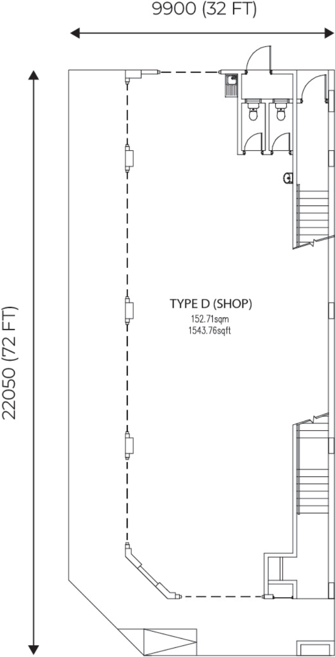
GROUND FLOOR
