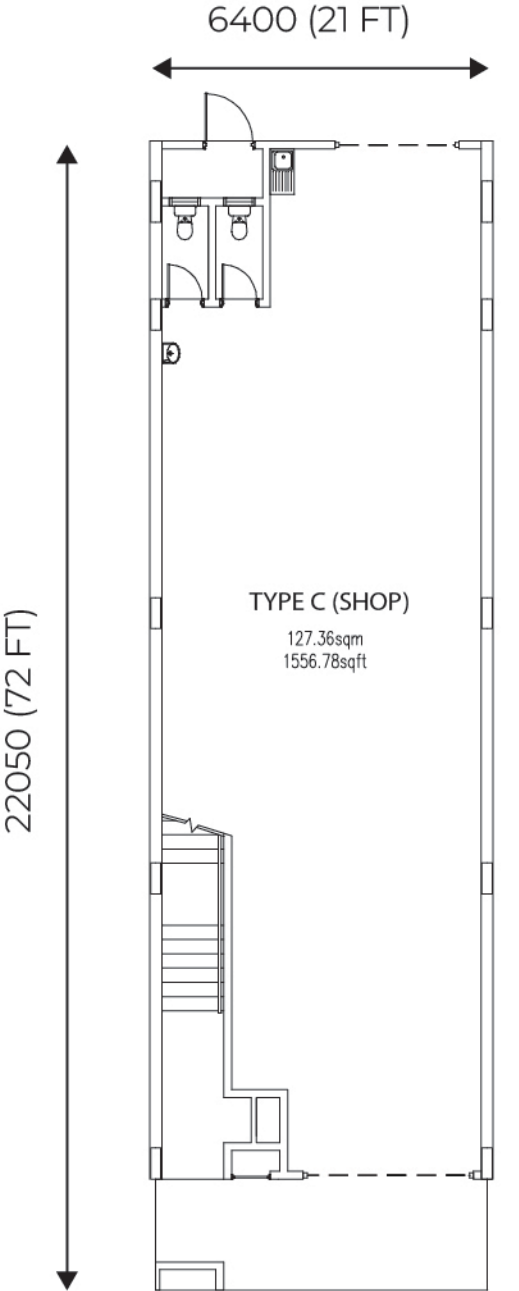
GROUND FLOOR
